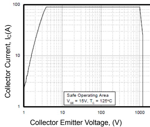
Figure 16. Turn-Off SOA
