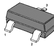
1.BASE 2.EMITTER 3.COLLECTOR TO-236 Plastic Package
