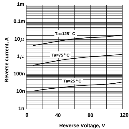
Reverse Characteristics
